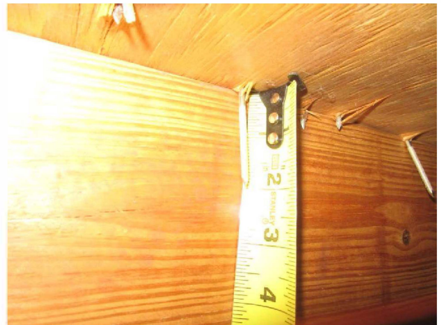
Roof Deck Attachment - 8d Nails
